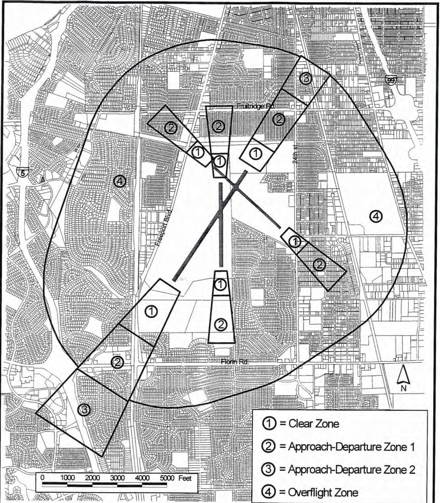
Figure 11 Sacramento Executive Airport Safety Zones
