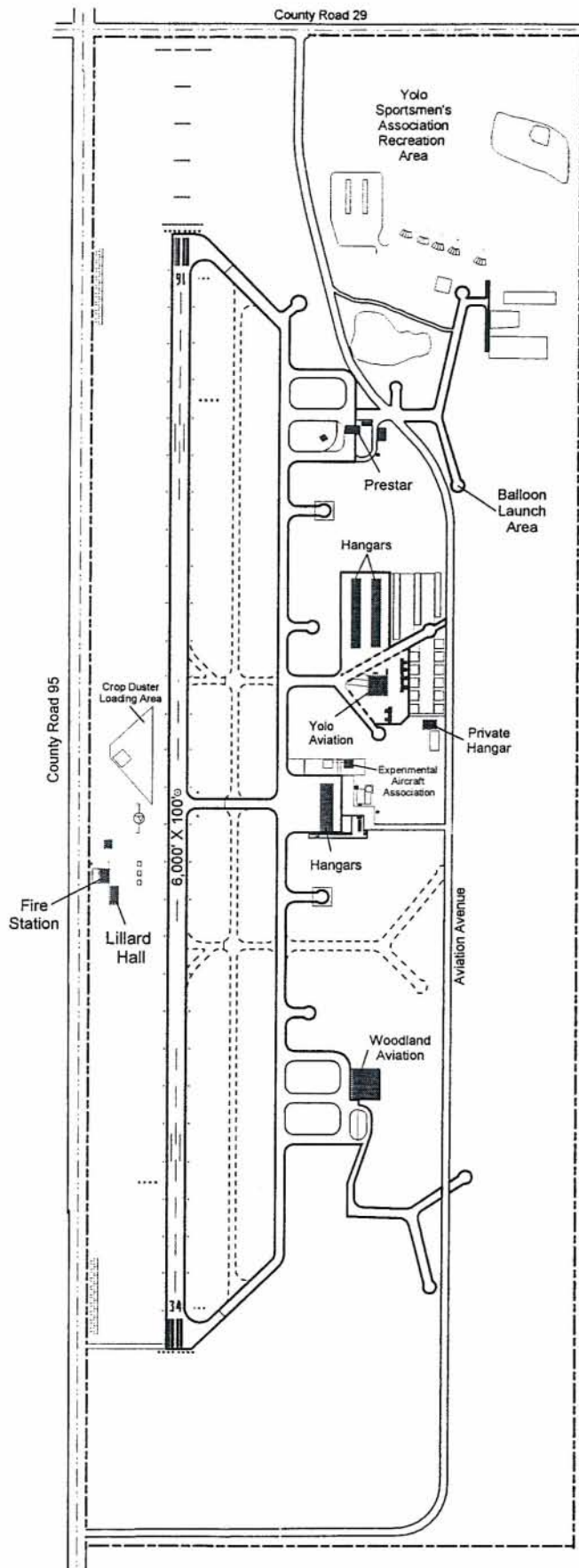
Figure 2 Airport Layout
