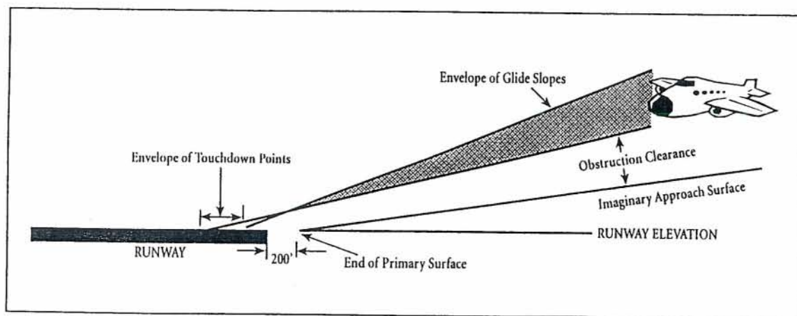
FIGURE 3 OBSTRUCTION CLEARANCES PROVIDED BY FAR PART 77 IMAGINARY SURFACES
