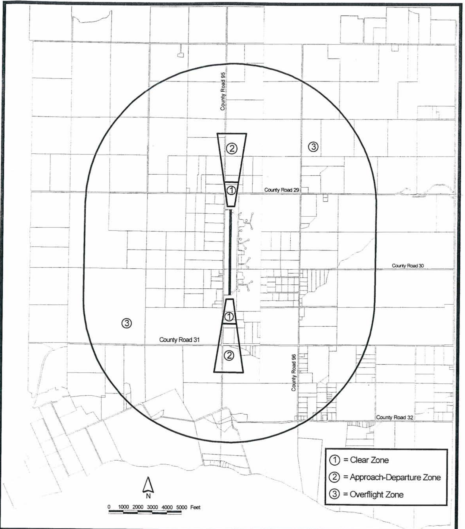
Figure 10 Yolo County Airport Safety Zones
